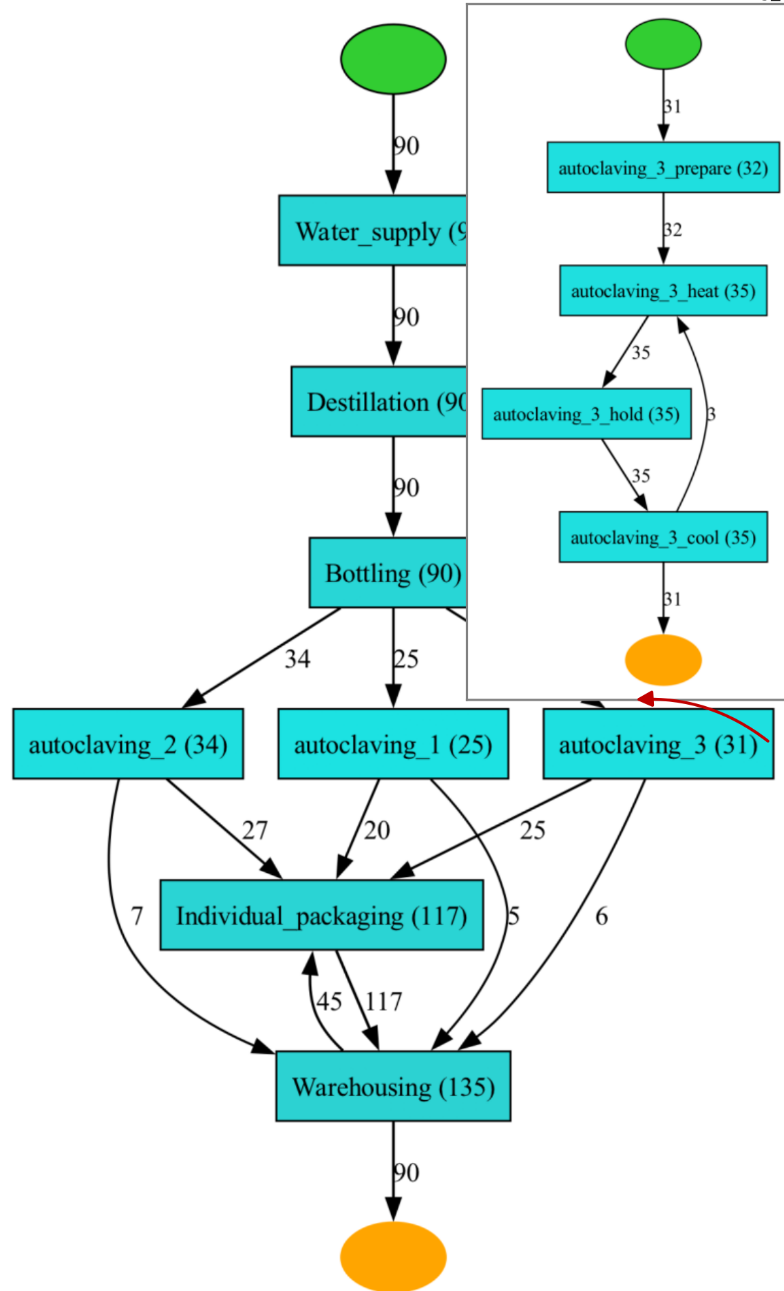
Material flow — stations, Autoclaving split into machines
