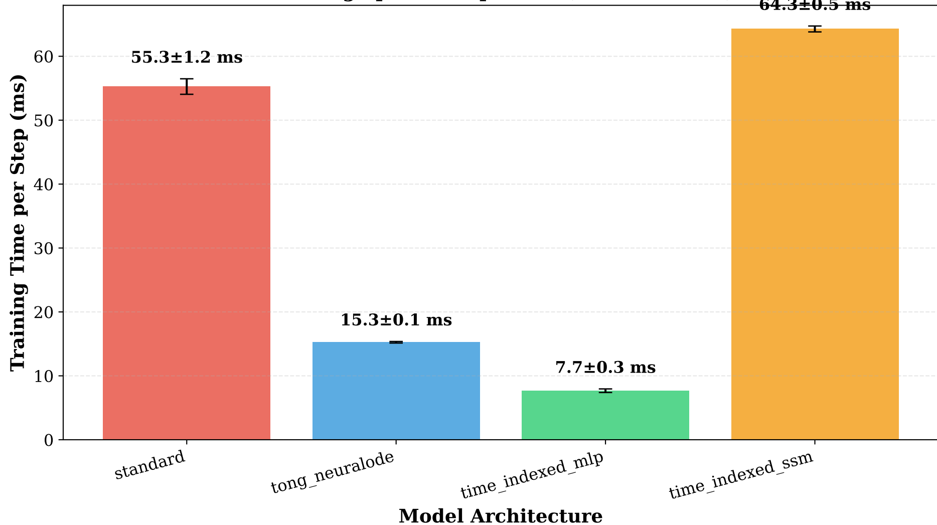
Training Speed Comparison (lower is better)
