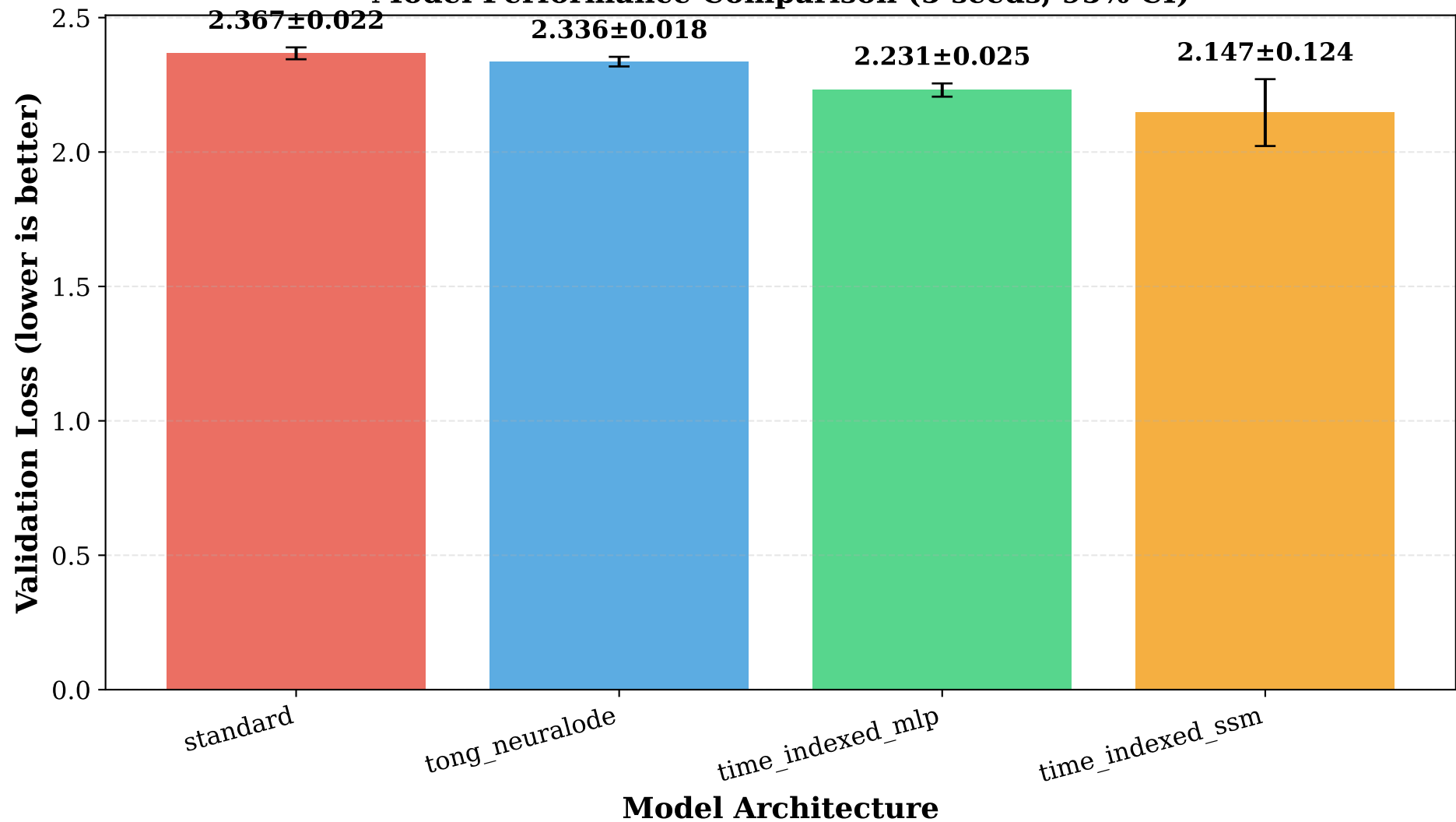
Model Performance Comparison (5 seeds, 95% CI)
