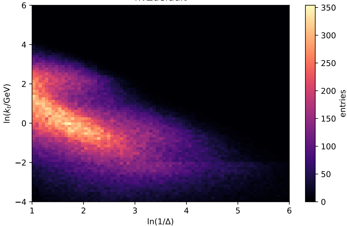
Lund plane for hvZdefault
