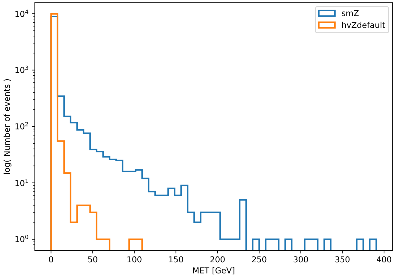
Missing transverse energy at truth level
