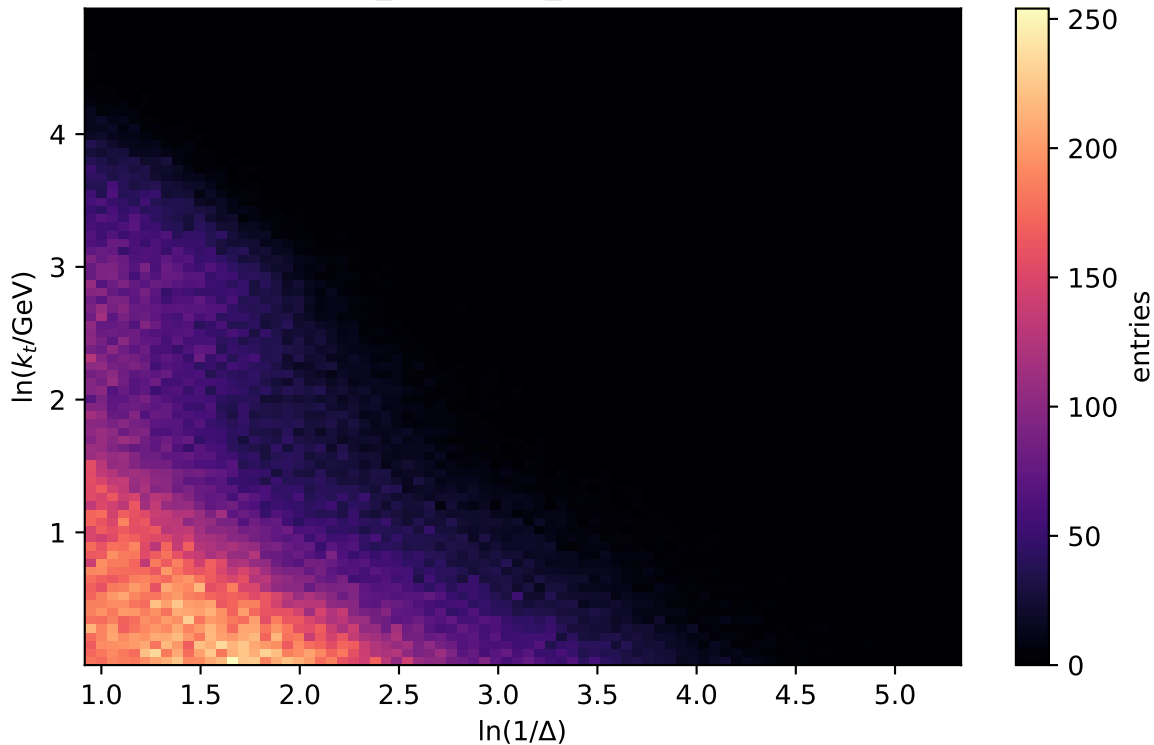
Lund plane for hvZ_23m1000_Lambda10
