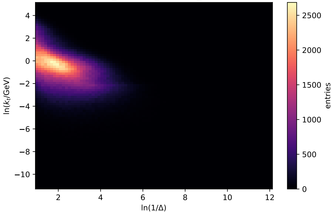
Lund plane for hvMihoko_101m20_111m10_113m25
