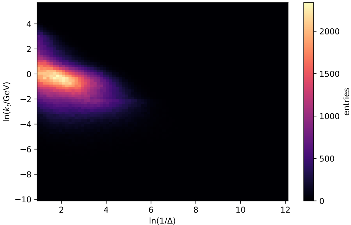
Lund plane for hvMihoko_101m40_111m10_113m25
