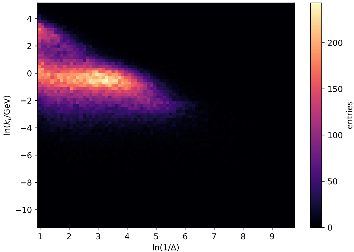
Lund plane for hvMihoko
