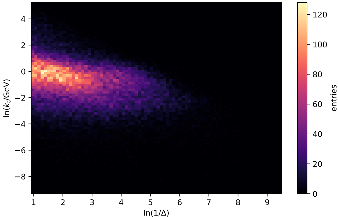
Lund plane for hvgg2DM_hardQCDnotset
