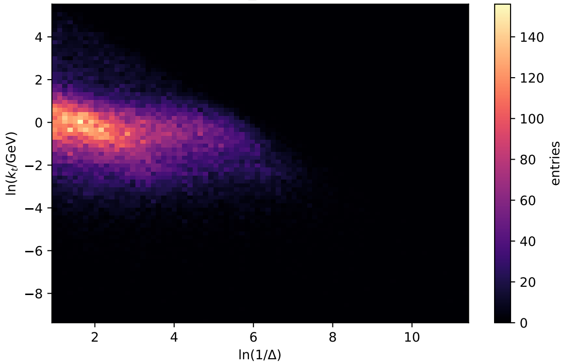
Lund plane for hv gg 2DM_hardQCDon
