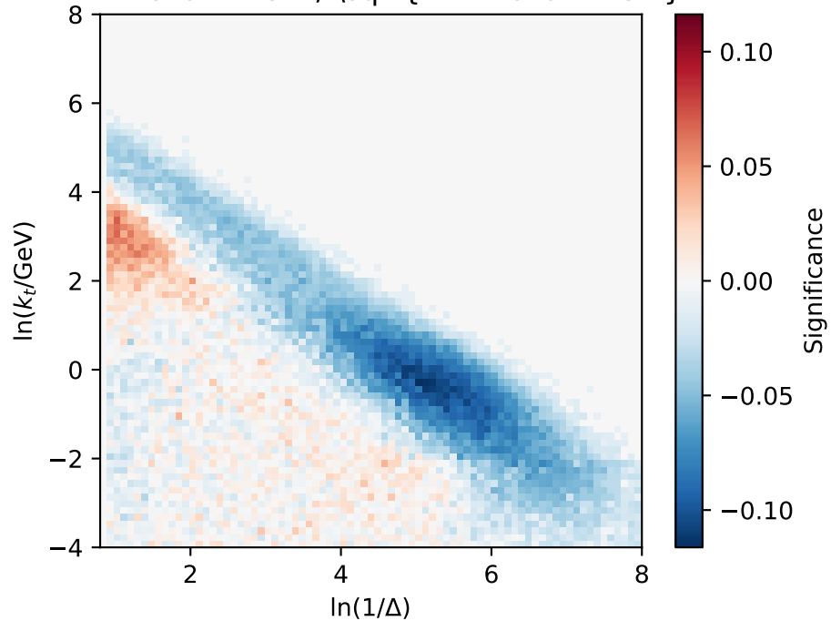
h \nu Mihoko - h \nu SM / \sqrt{\text{h}\nu\text{Mihoko} + \text{h}\nu\text{SM}}
