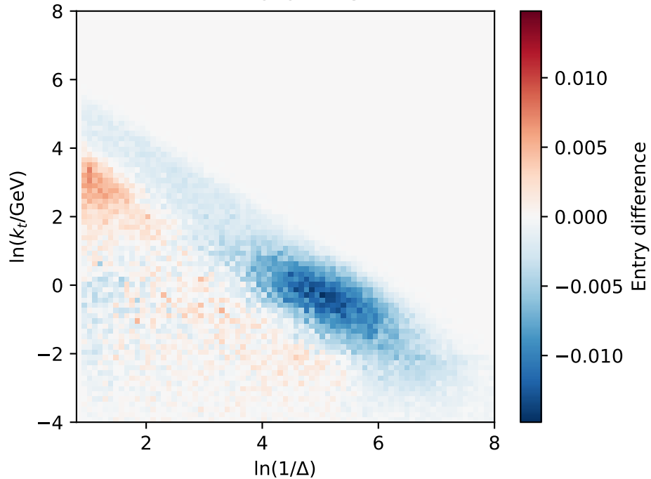
h \nu Mihoko - h \nu SM
