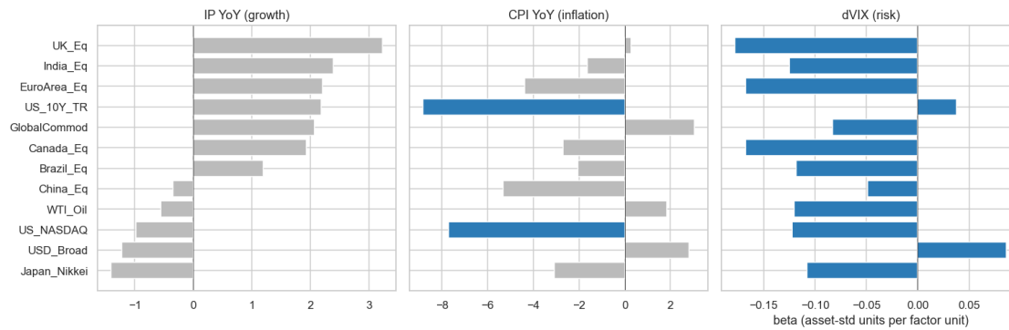
In-sample factor loadings (blue = |t| \geq 2 with HAC SE)
