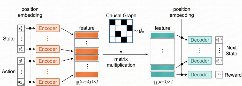
Figure 1: Schematic of the structural transition model used to generate next-state and reward targets for perturbed states.
