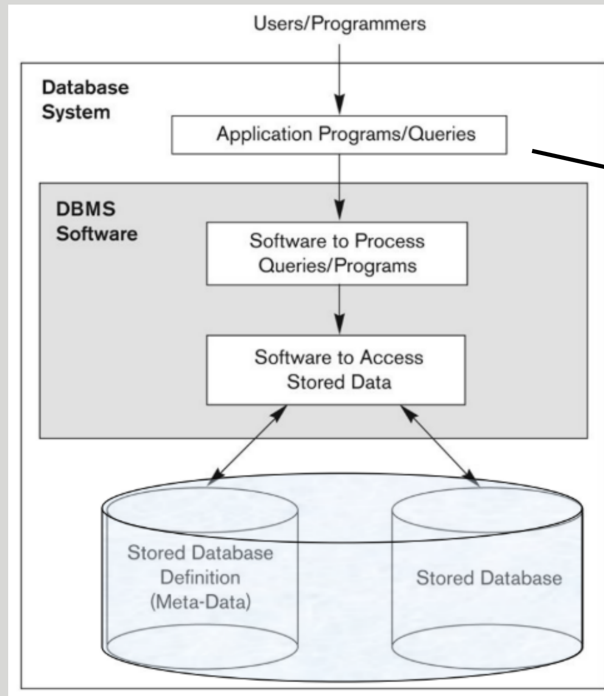
Fig: Simplified Database System Environment
