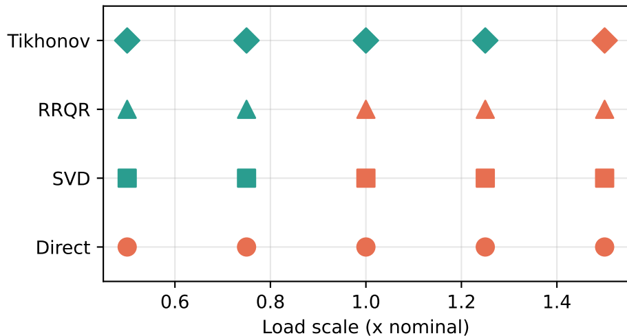
IEEE 13-bus: solver convergence vs. load (green = converged, red = failed)
