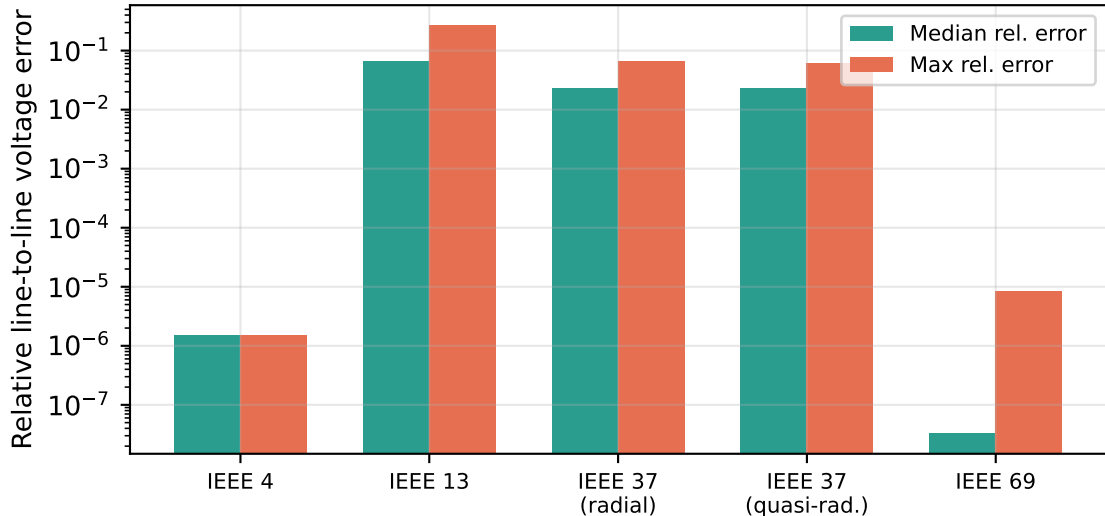
OpenDSS cross-validation error by feeder
