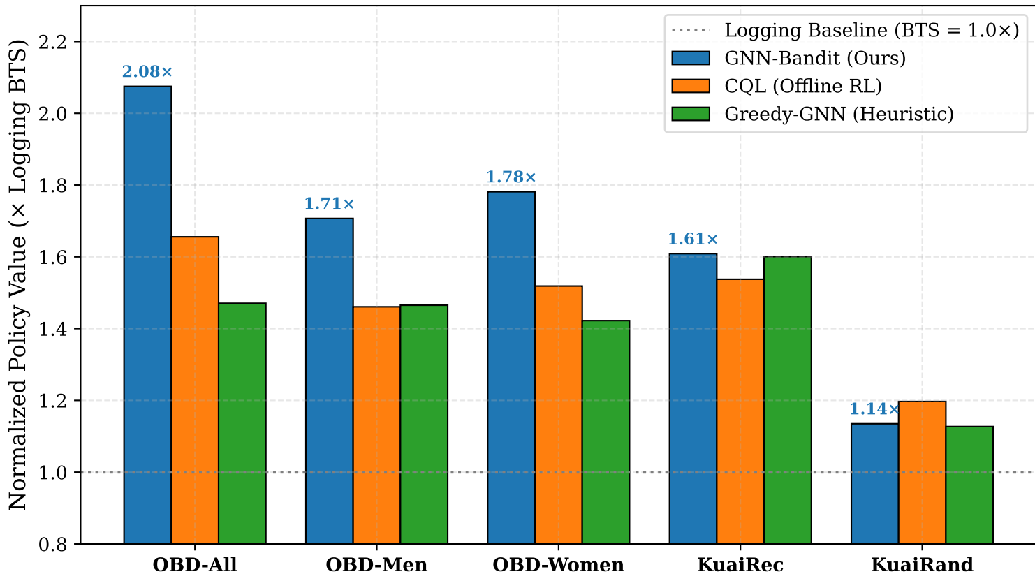
Cross-Dataset Empirical Superiority across Diverse Domains
