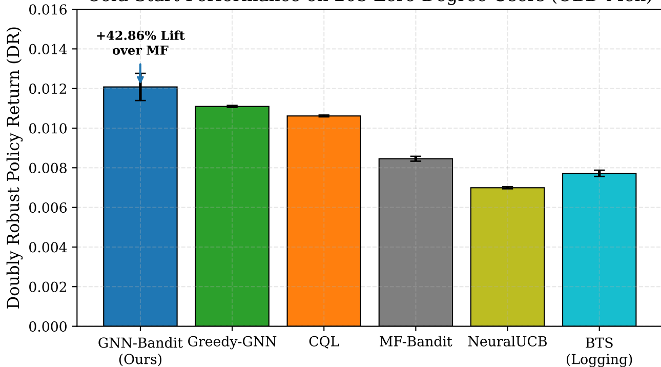
Cold-Start Performance on 205 Zero-Degree Users (OBD-Men)
