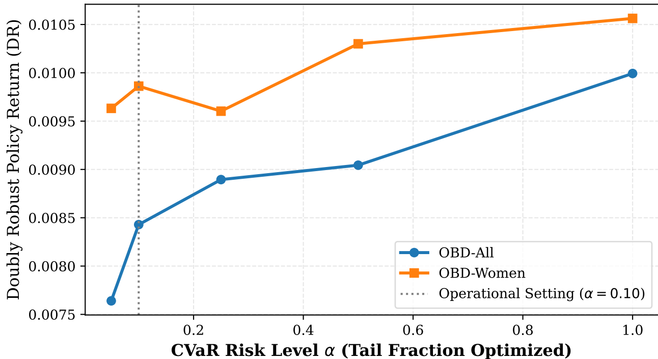
Risk-Averse Safety Trade-off Curve Across Quantile Cutoffs \alpha
