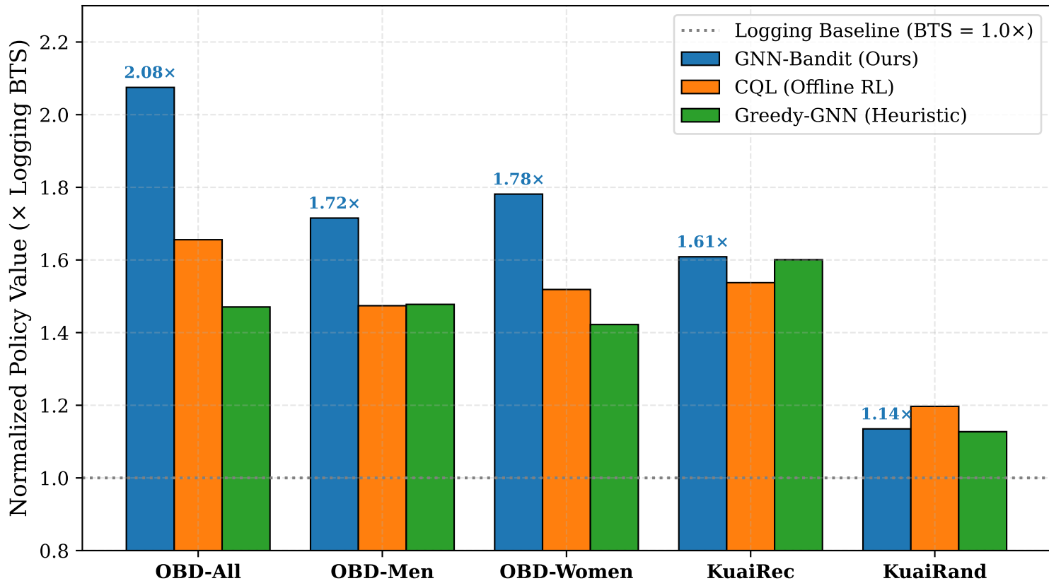
Policy Value Relative to Logging Policy across Datasets
