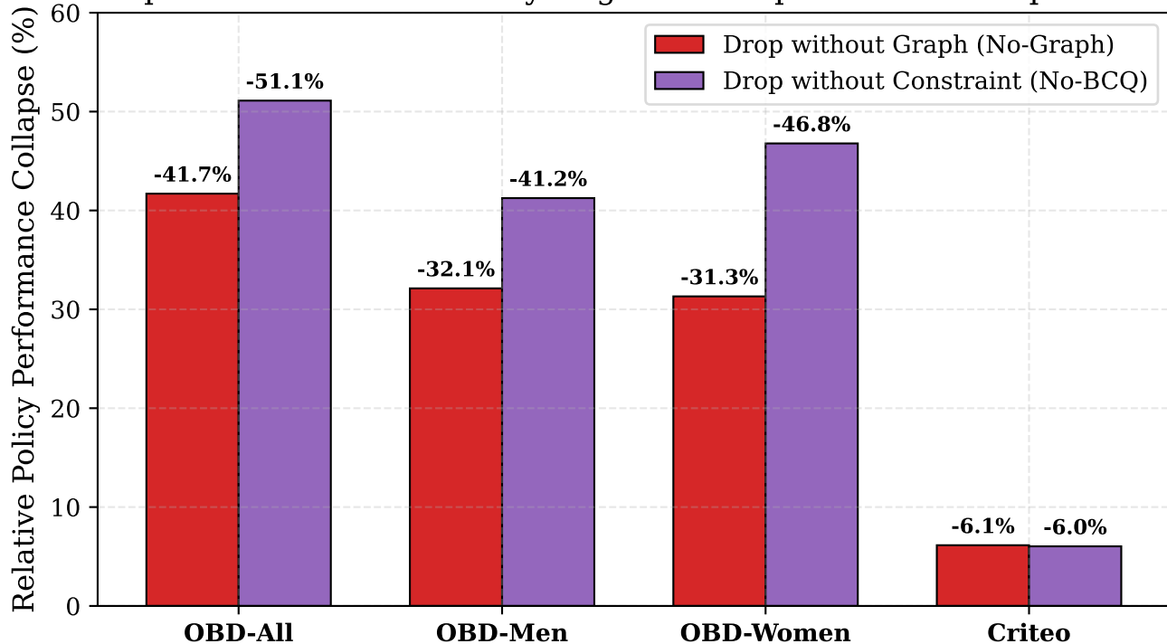
Component-Wise Ablation: Synergistic Collapse without Graph or BCQ
