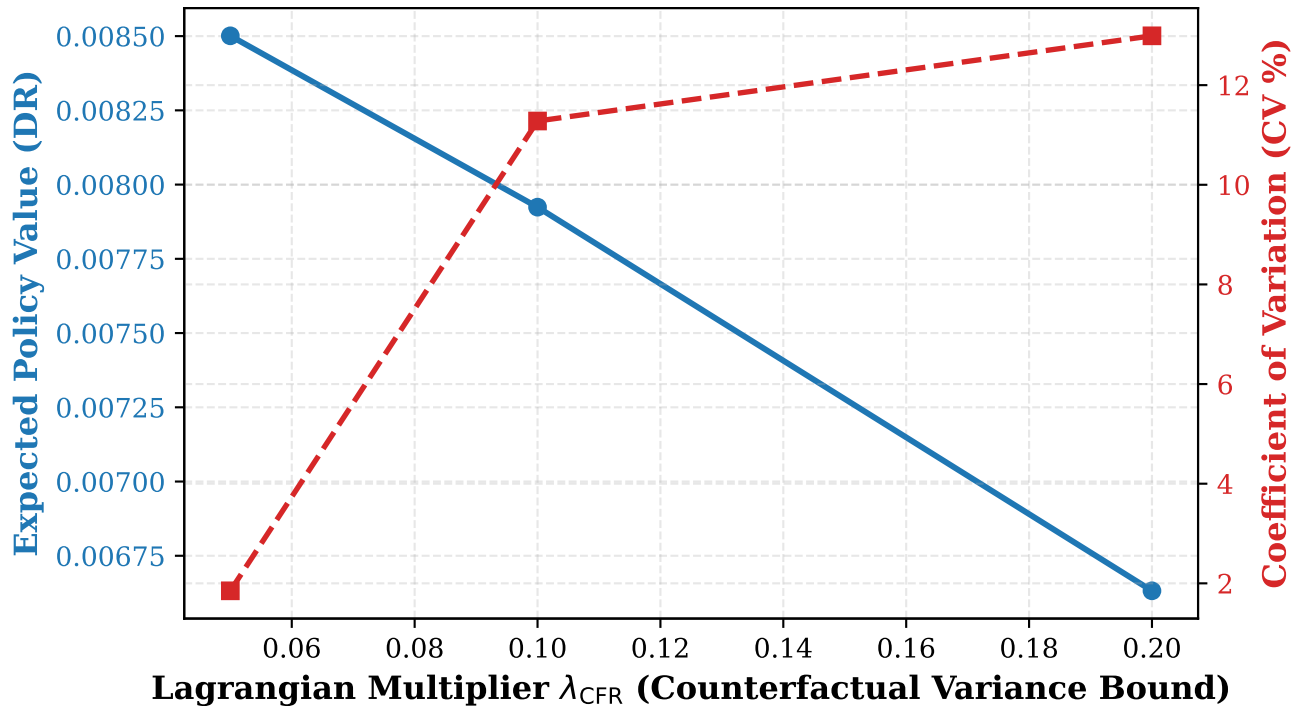
Lagrangian Pareto Frontier: Policy Value vs. Counterfactual Variance
