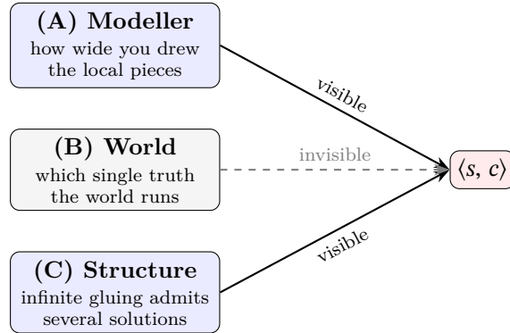
Figure 4: Three sources of freedom and what the two numbers can see. (A) and (C) reach \langle s, c \rangle ; (B), the world’s single hidden pick, does not — and that blindness is the correct behaviour, because the truth value describes the set, not the pick. (A) is freedom you declared ; (C) is freedom the structure produces emergently — different origins, both visible.
