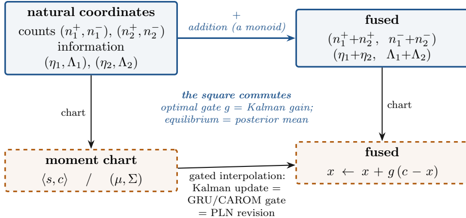
Figure 7: Fusion is addition; charts are shadows. Three rules invented independently in three literatures — Kalman filtering, gated recurrence, probabilistic-logic revision — are one operation, and it is only nonlinear because the moment chart is.
