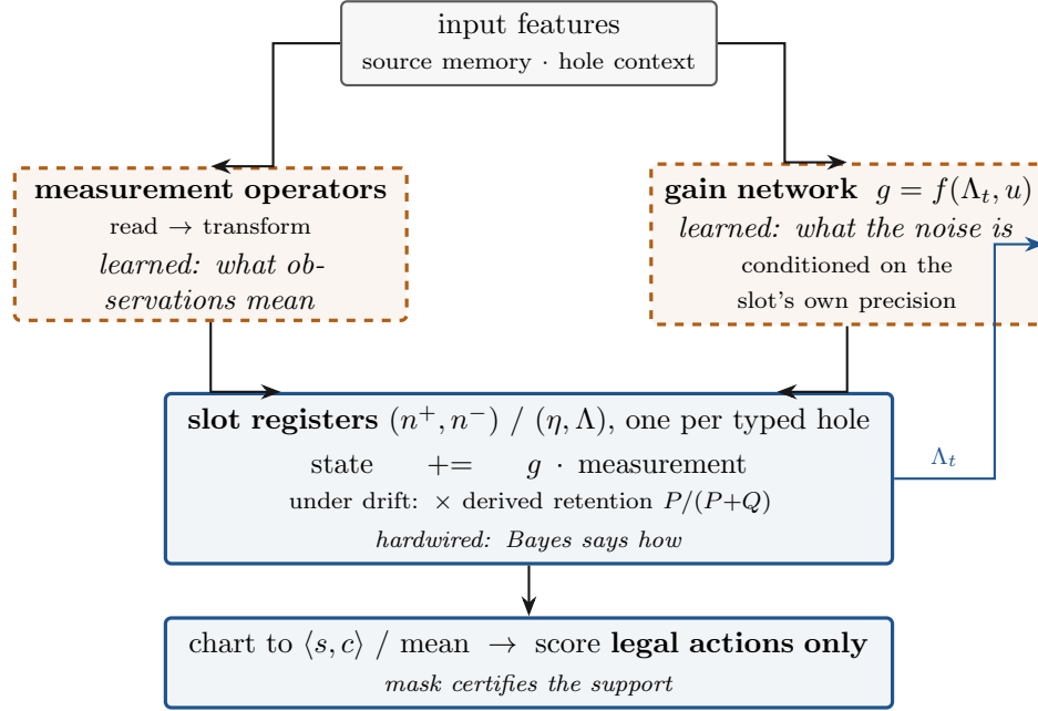
Figure 8: The cell the theorems license. Learning concentrates where Bayes is silent — in the measurement maps and the gain schedule — while fusion itself is the addition Bayes prescribes. The precision register feeds the gain network, which is what makes selectivity possible; the readout can only rank actions the checker already admits.
