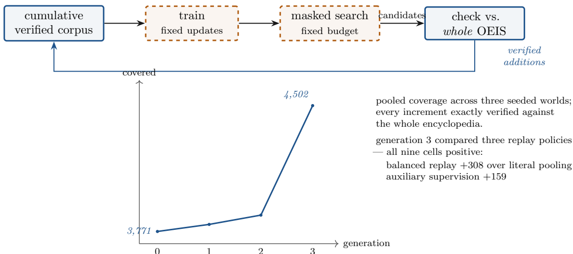
Figure 9: The loop compounds. At literal pooling the model’s own discoveries carry 0.24% of sampling mass and the loop starves on the signal it exists to generate; balanced replay is what makes self-improvement visible.
