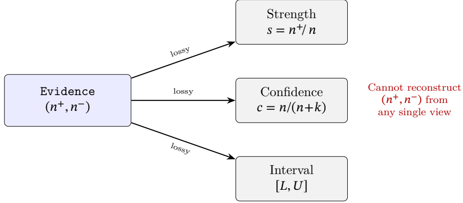
Figure 8.1: Truth-value views are projections from Evidence. Strength, confidence, and interval bounds each discard information. A fixed- k strength-confidence pair can recover binary counts in the idealized scalar model, but no single scalar view reconstructs the full evidence state.
