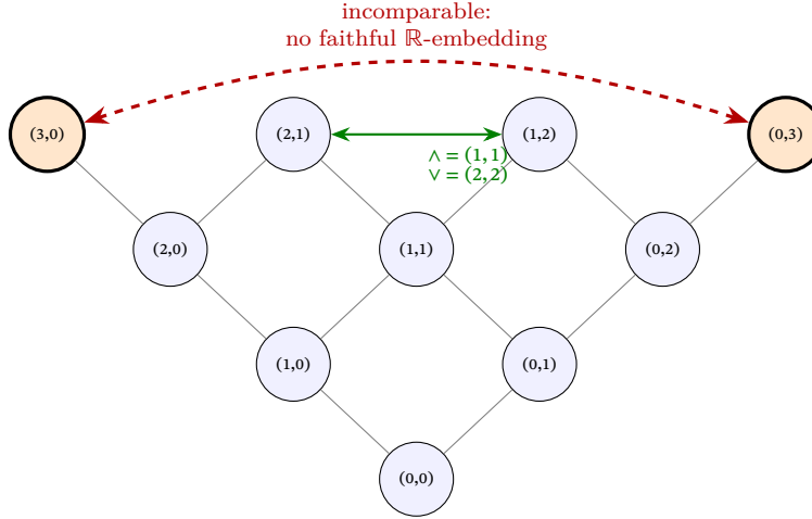
Figure 6.1: Hasse diagram of the Evidence lattice (first four levels). The information ordering is componentwise: (a^+, a^-) \leq (b^+, b^-) iff both coordinates are \leq . Orange nodes (3,0) and (0,3) are incomparable—no single real-valued function preserves the full ordering (the “totality gate”). The green link shows meet and join: \wedge((2,1), (1,2)) = (1,1) , \vee = (2,2) .
