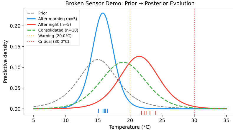
Figure 21.1: Broken sensor demo. Gray dashed: prior predictive. Blue: posterior after morning shift ( \sim 16^\circ\text{C} ). Red: posterior after night shift ( \sim 22^\circ\text{C} ). Green dashed: consolidated posterior. Data tick marks on the x-axis. Sleep consolidation is verified: sequential and batch processing yield the same posterior.
