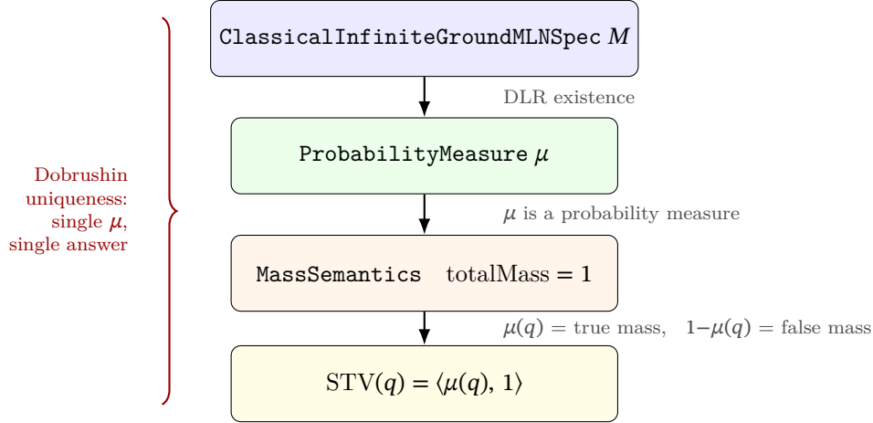
Figure 17.2: The infinite MLN \rightarrow WM semantic pipeline. Each arrow is a Lean definition or theorem; the left brace marks the scope of the Dobrushin uniqueness guarantee. Under uniqueness, the query credal width is zero, so the confidence-like width-complement is 1; the separate 1 - \mu(q) quantity is false mass, not confidence.
