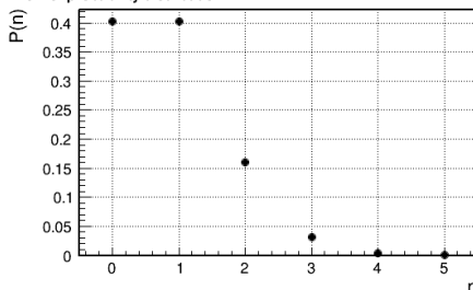
Binomial probability distribution
