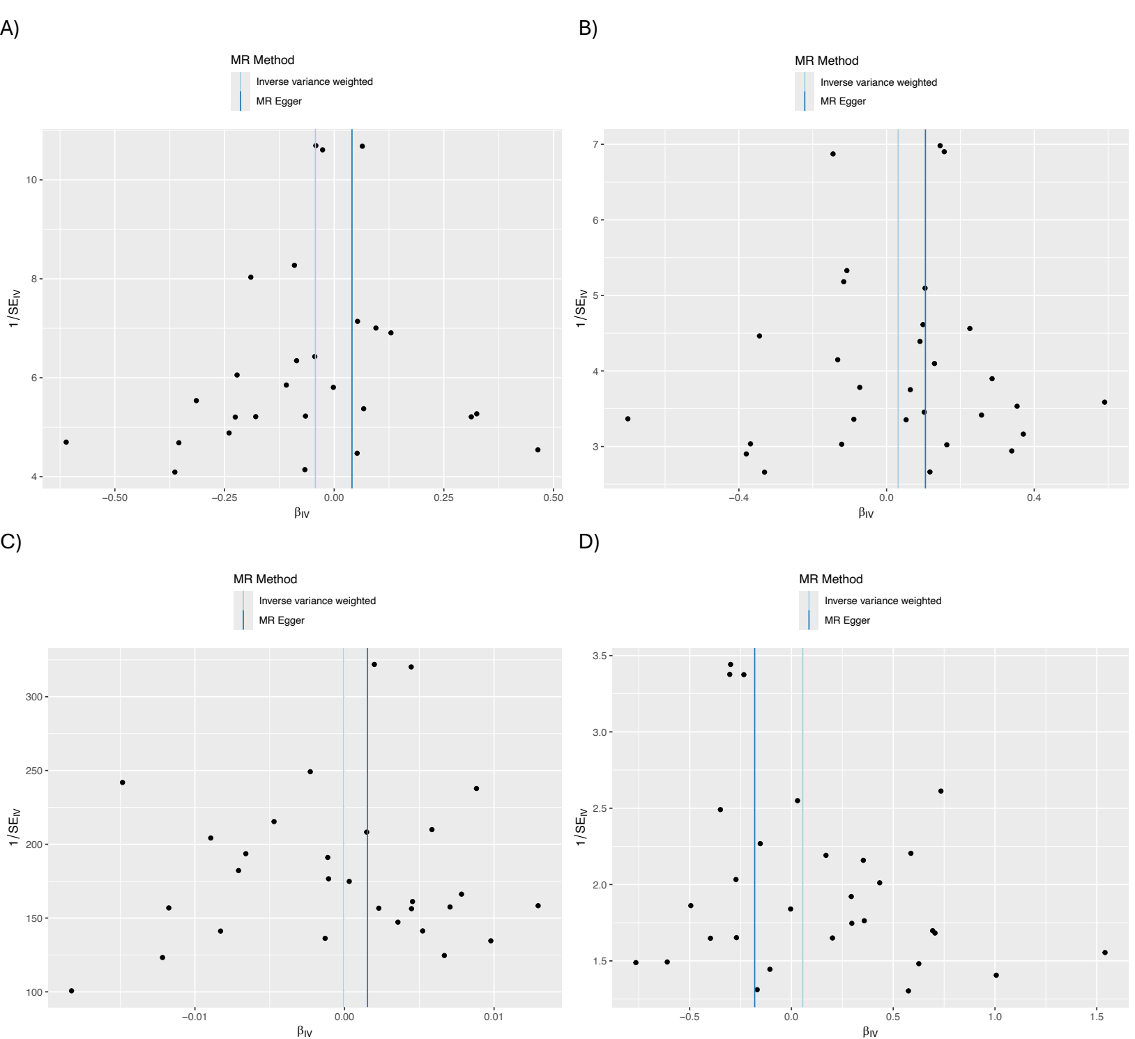
Figure S1. Funnel plots of SNP-specific causal estimates ( \beta_{IV} ) against precision ( 1/SE_{IV} ) assessing horizontal pleiotropy in Mendelian randomization analyses of endometriosis on psychiatric outcomes. Panels: (A) Mood disorders; (B) Behavioural syndromes; (C) Anxiety disorders; (D) Schizophrenia.
