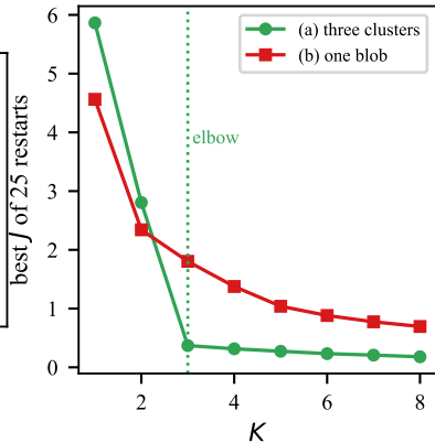
(c) J versus K
