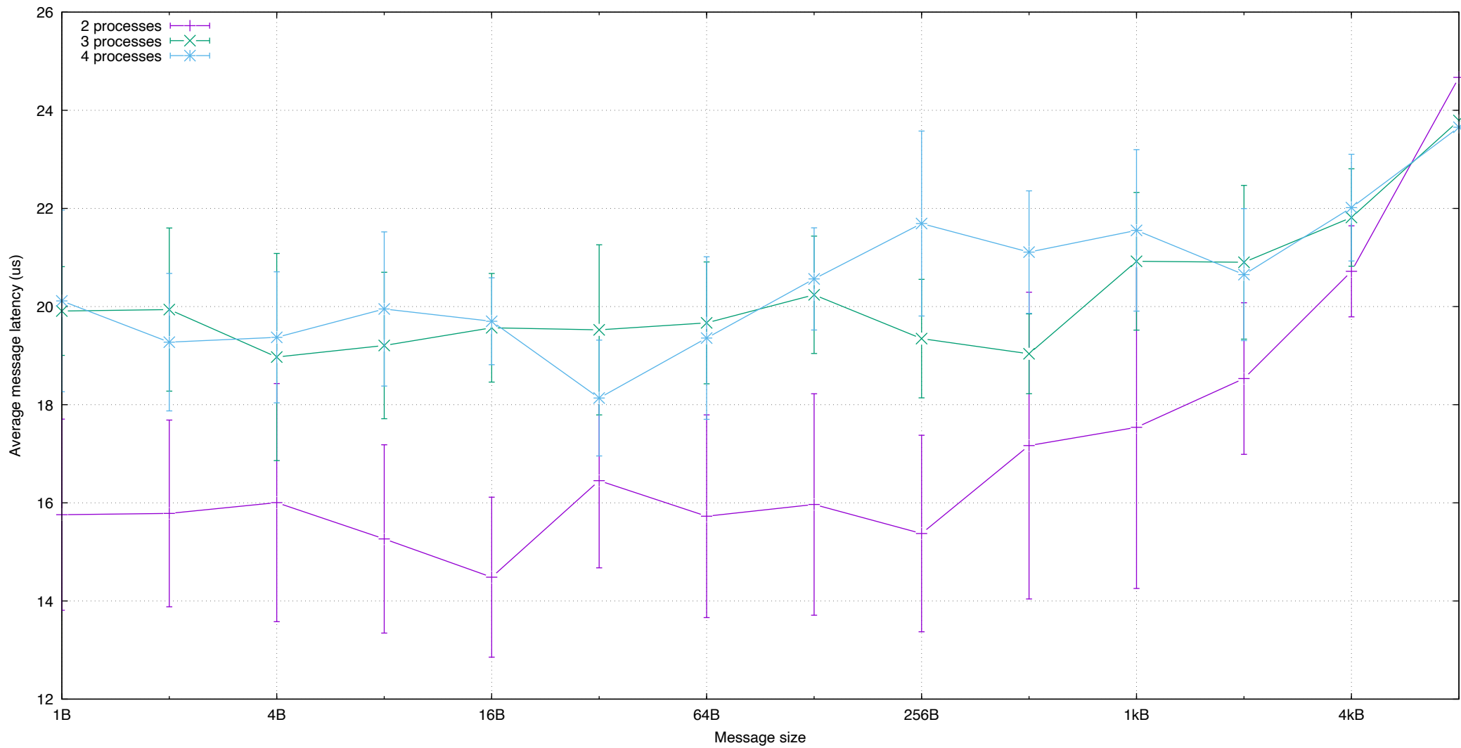
All-to-All IPC Latency vs Message Size
