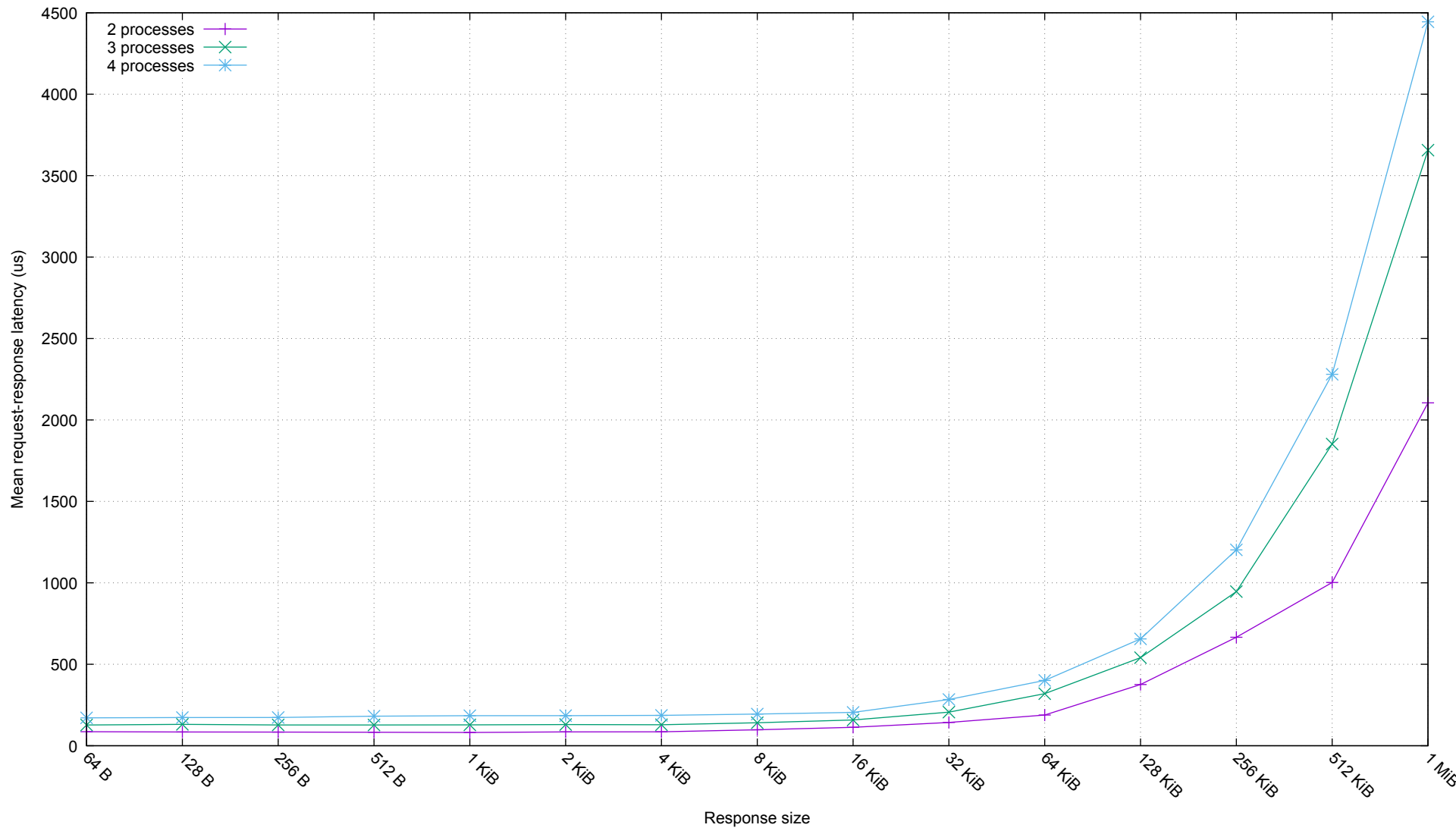
Distributed DB Benchmark: Latency vs Response Size
