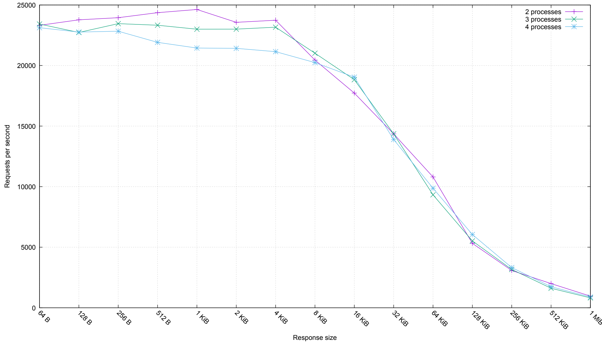
Distributed DB Benchmark: Requests per Second vs Response Size
