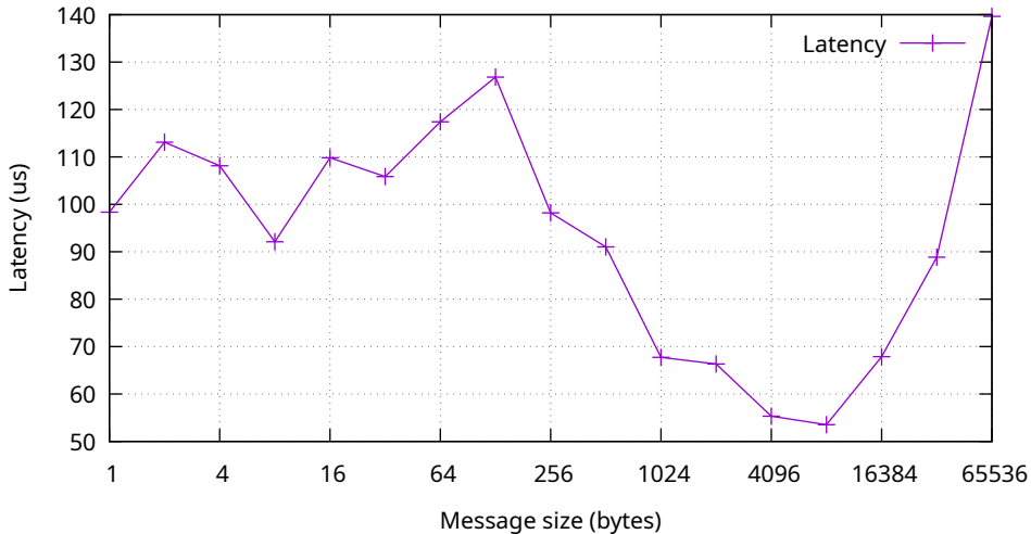
IPC Roundtrip Latency vs Message Size
