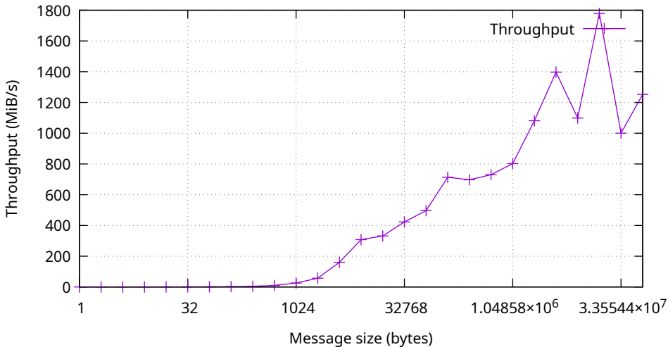
IPC Throughput vs Message Size
