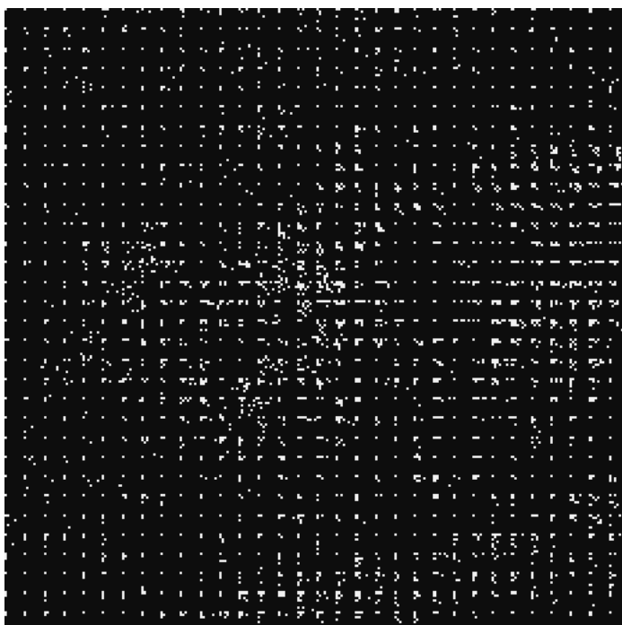
Block DCT (8×8)
