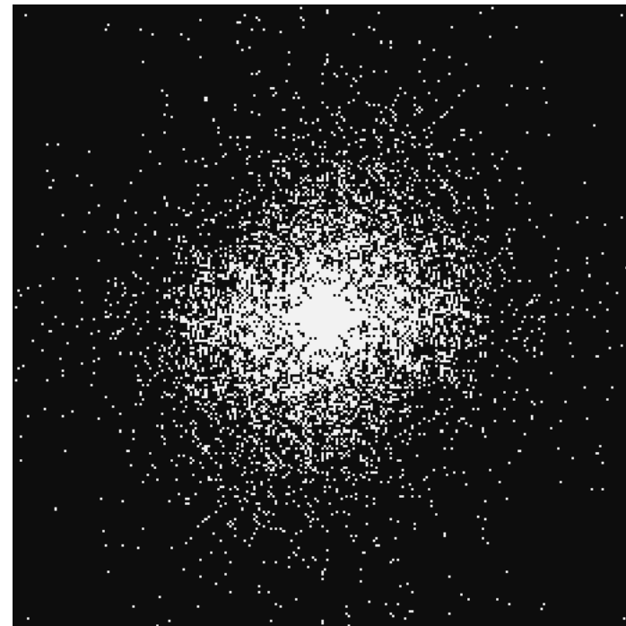
10% kept (k=6554)
