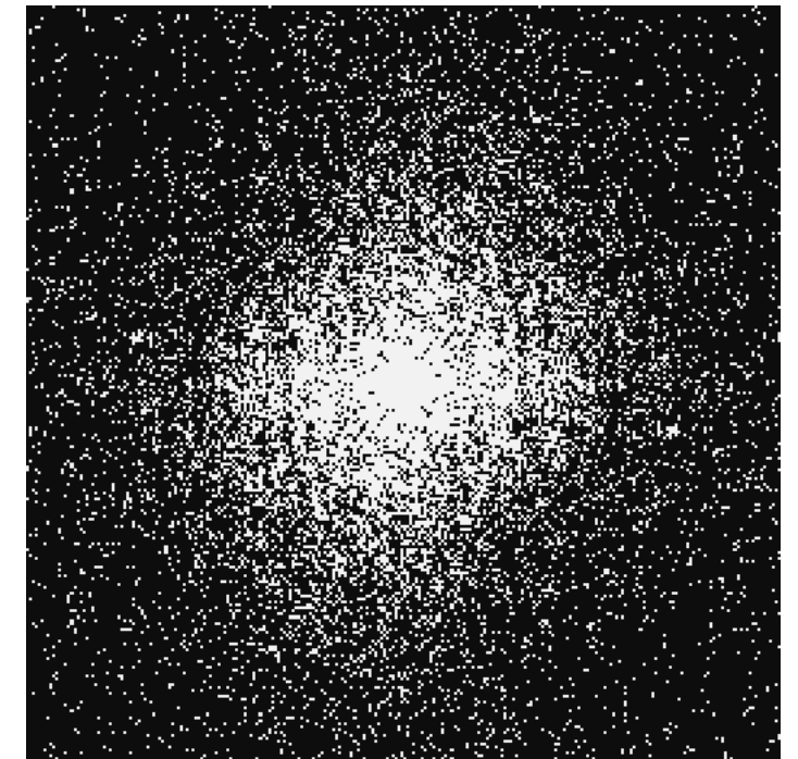
20% kept (k=13107)
