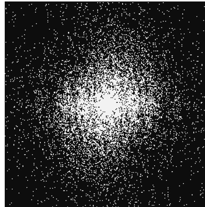
15% kept (k=9830)
