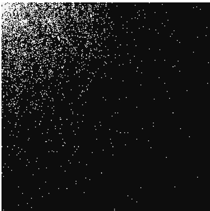
Classical DCT
