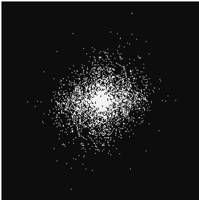
Classical FFT
