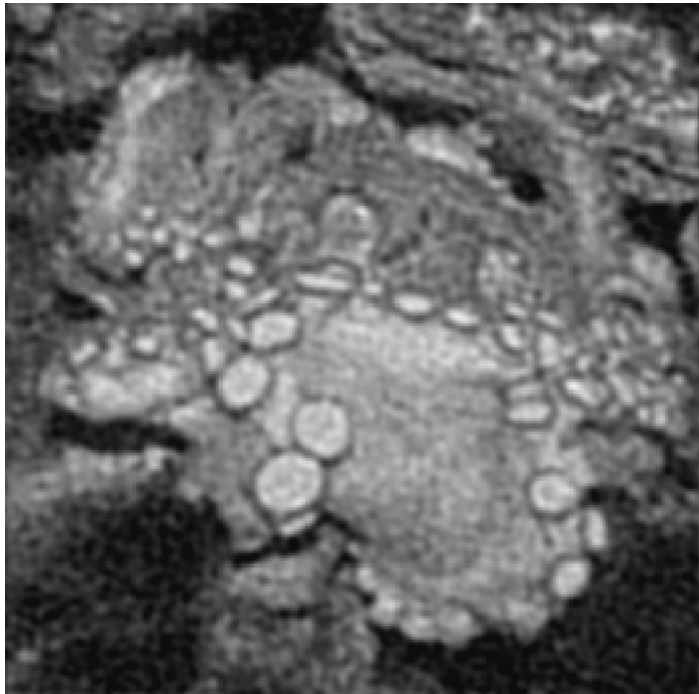
Classical FFT
