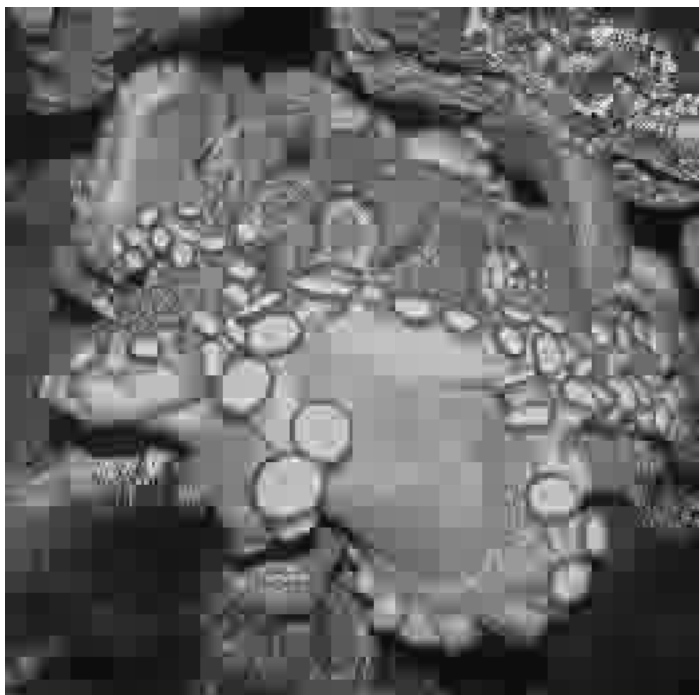
Block DCT (8×8)
