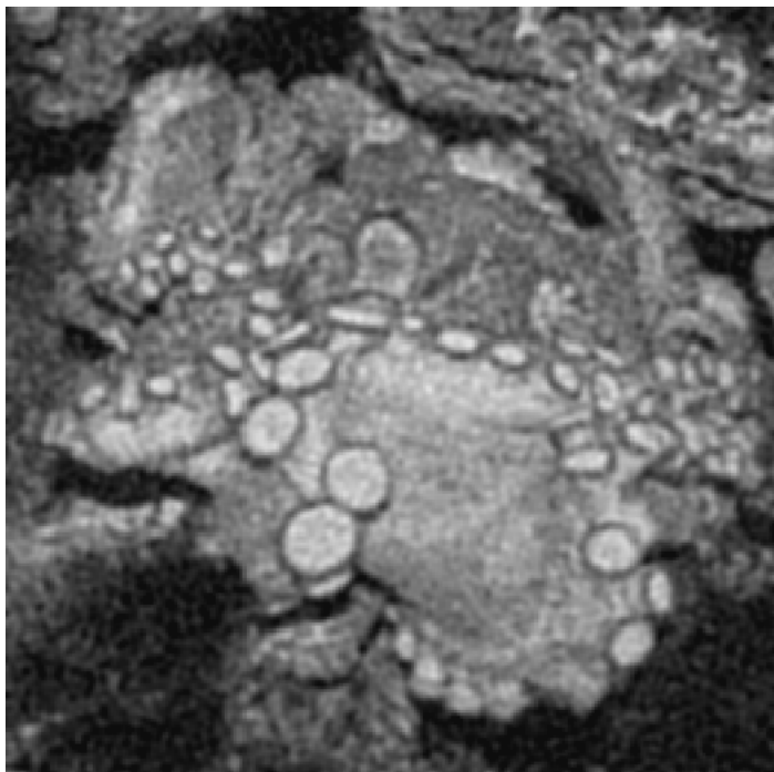
Classical DCT
