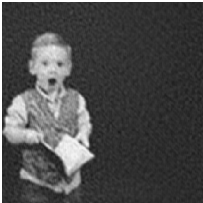
Classical FFT
