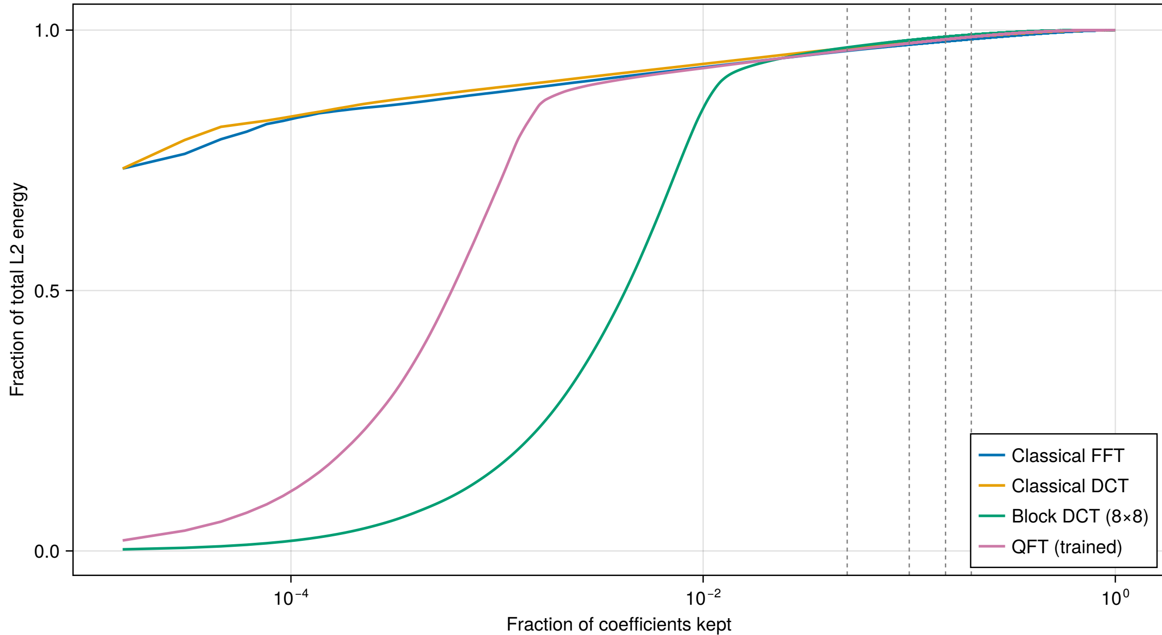
Energy captured vs. fraction kept — 0771.png
