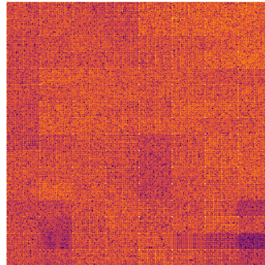
QFT (trained)
