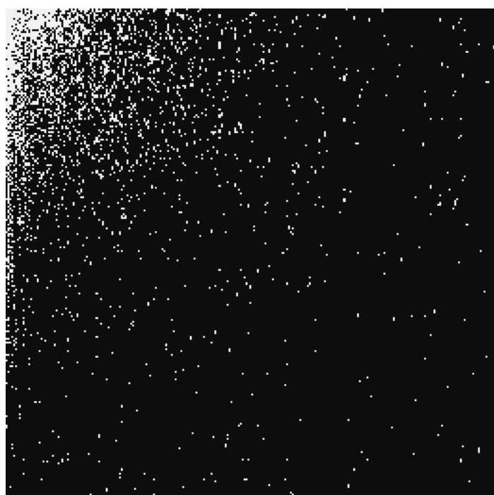
Classical DCT
