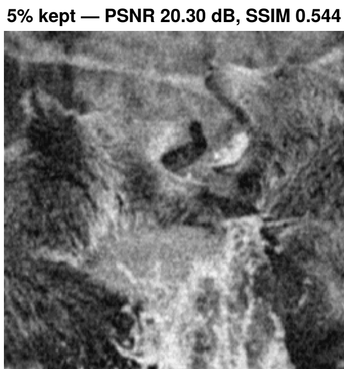
Classical DCT
