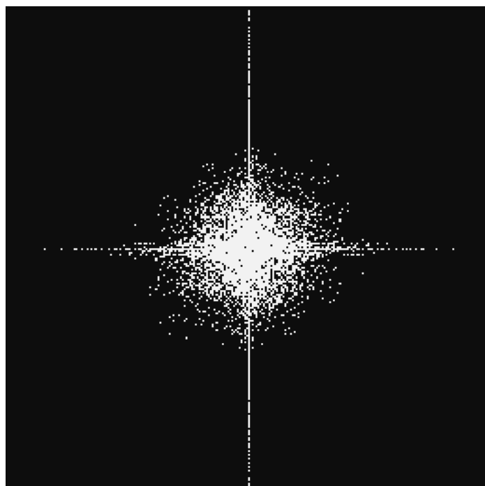
Classical FFT
