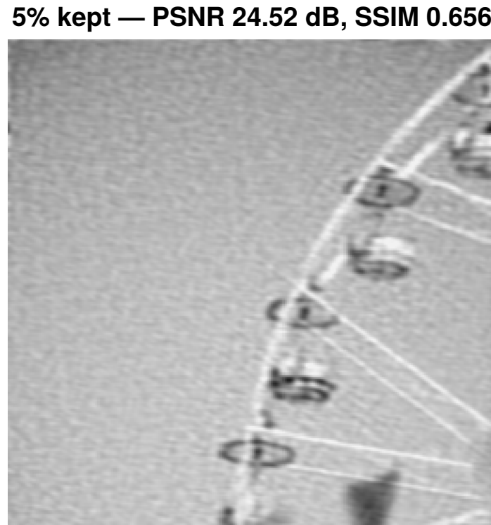
Classical FFT
