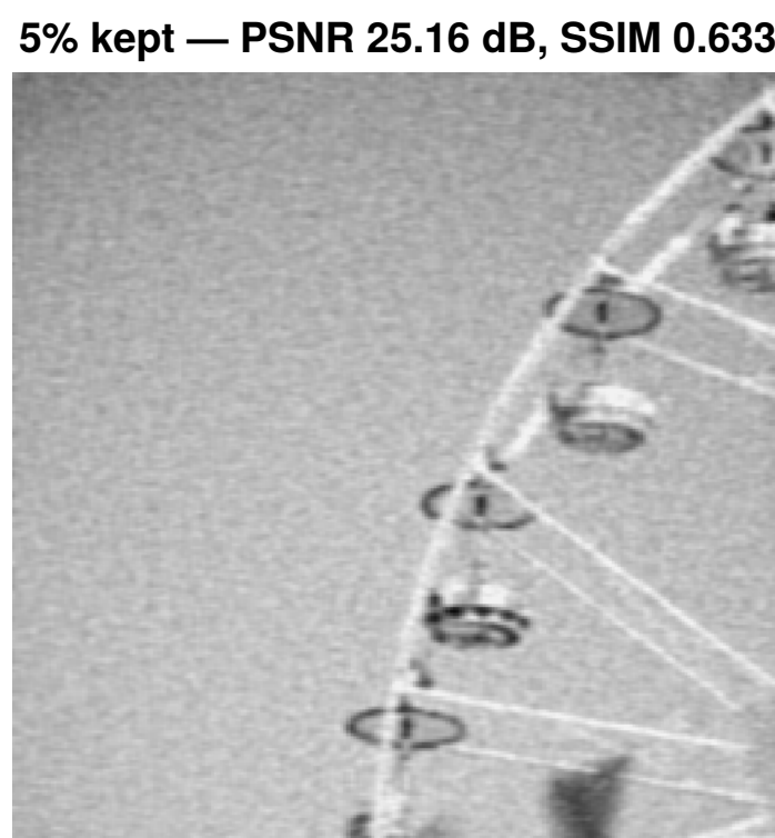
Classical DCT
