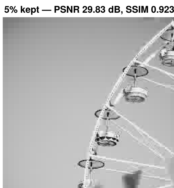
Block DCT (8×8)
