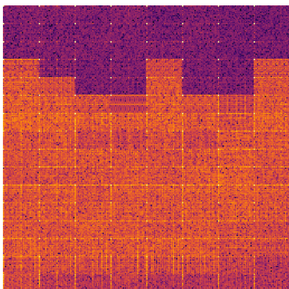
Entangled QFT
