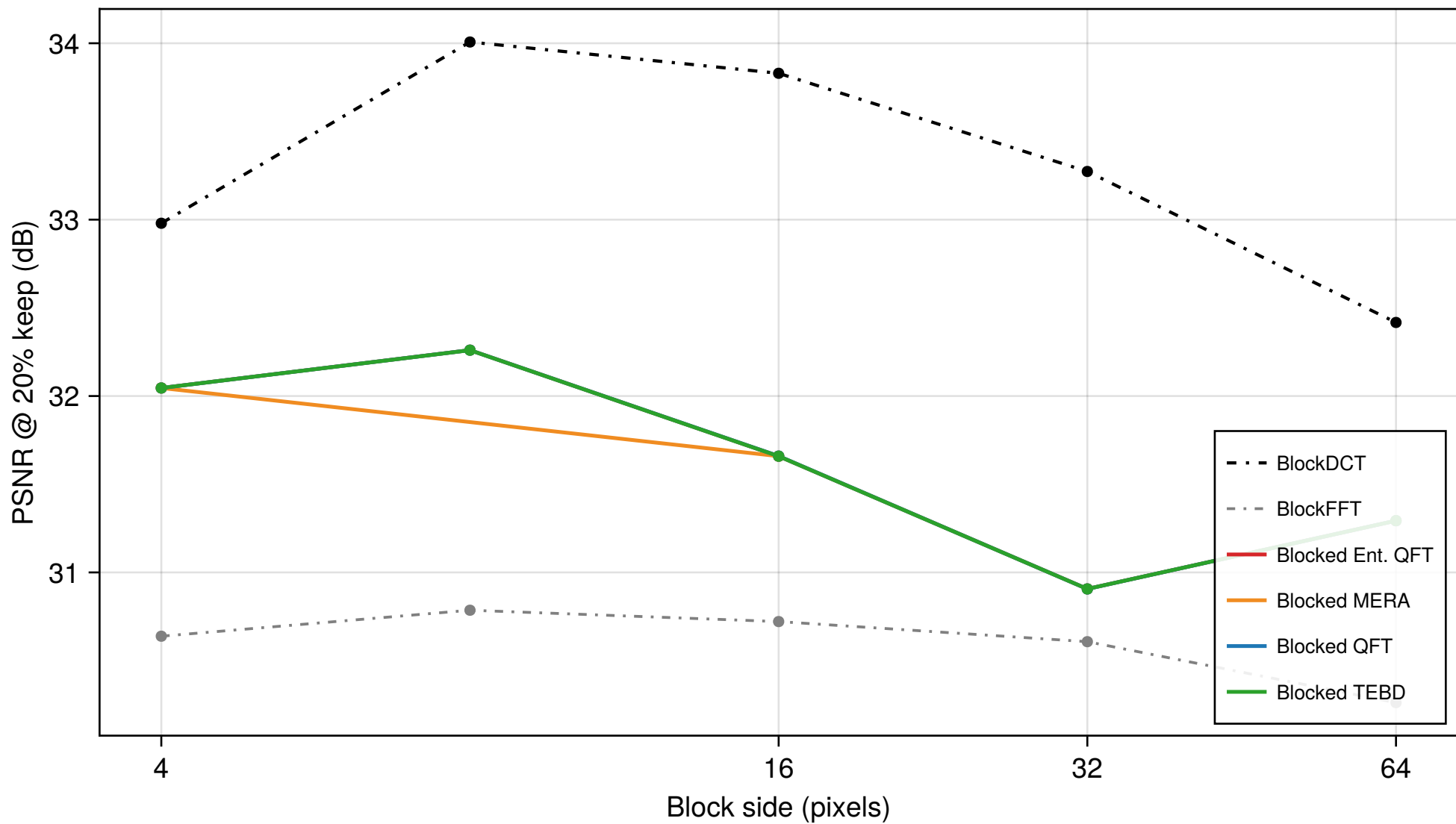
Block-size axis on DIV2K 256×256
