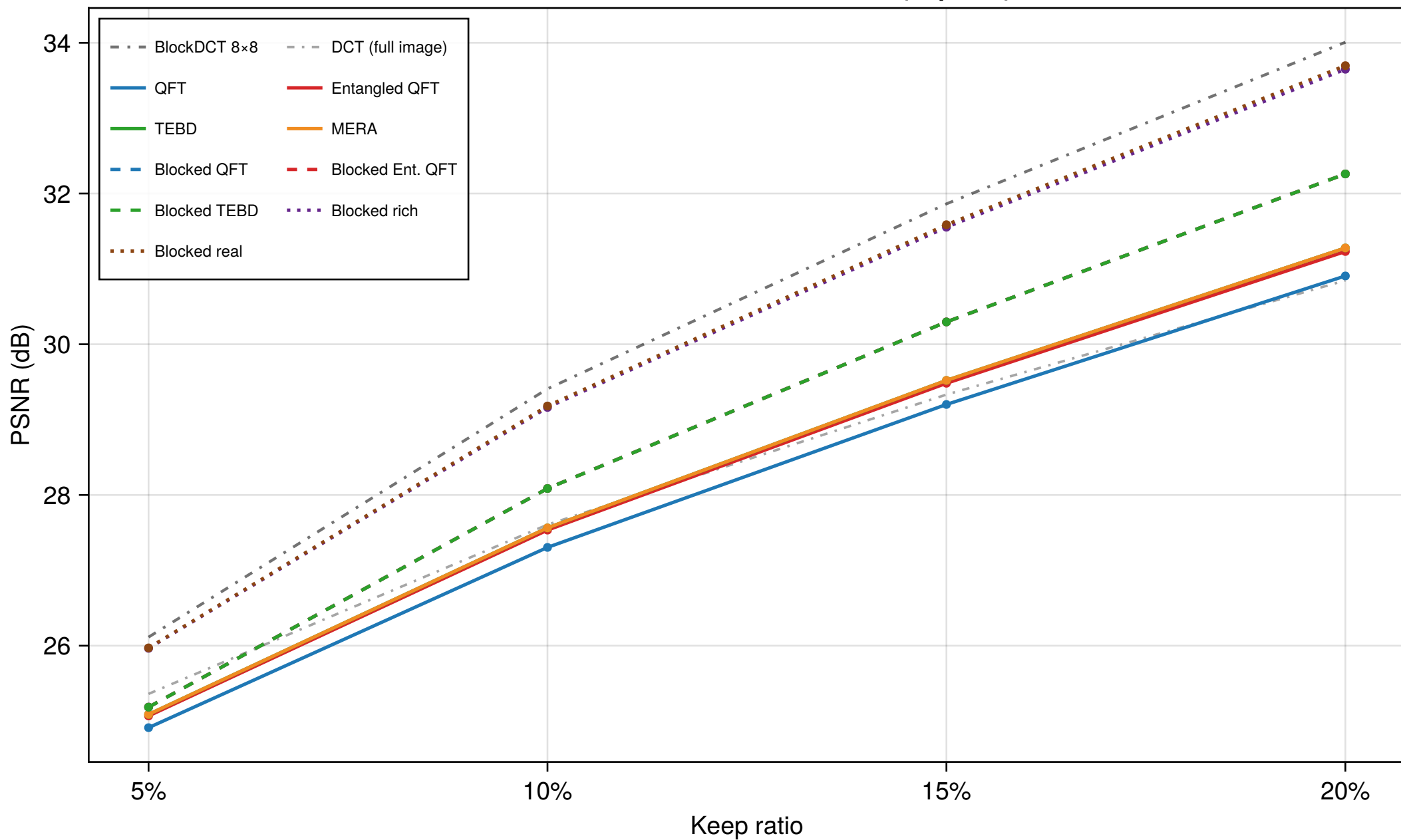
Basis variations on DIV2K 256×256 (8 qubits)
