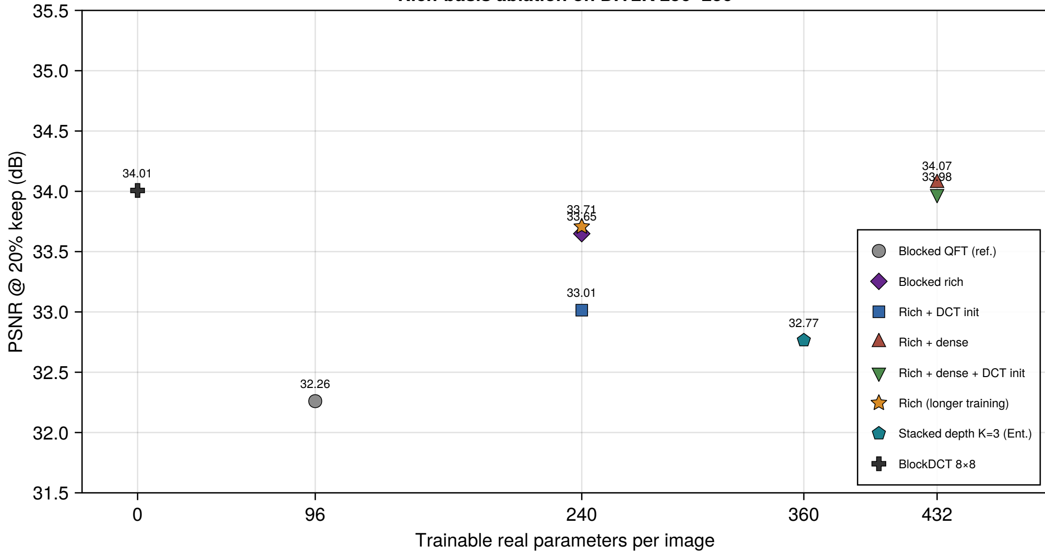
Rich-basis ablation on DIV2K 256×256
