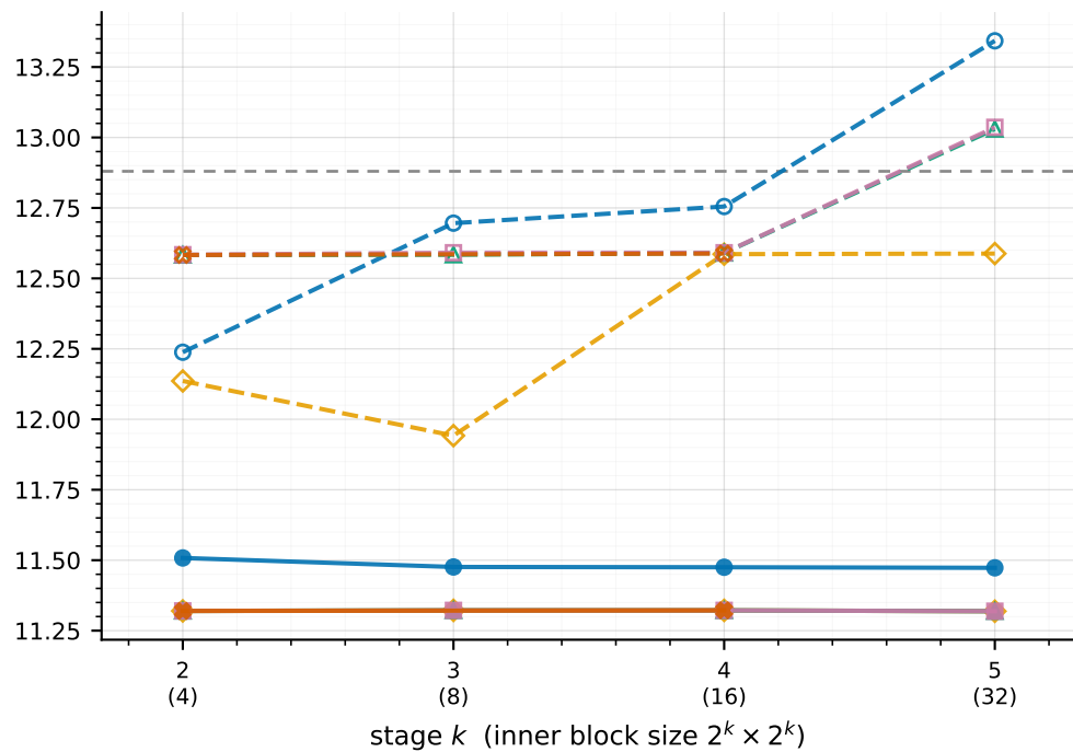
\rho = 0.01 (100 \times compression) · block-DCT-8 12.9 dB
