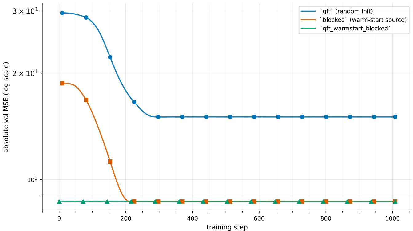
Figure 2: QuickDraw. Validation MSE per training step (log y). Same three curves as the DIV2K figure with smaller absolute scales (32×32 images, 1024 pixels, K = 102 ). Blue: qft random init ( 30 → 15). Orange: blocked warm-start source ( 19 → 8.7). Green: qft_warmstart_blocked again flat at the blocked floor (val MSE in [8.67, 8.68] throughout). Loss definition is the same form as DIV2K with K = 102 , summed over 1024 pixels, averaged over the 75-image validation split.
